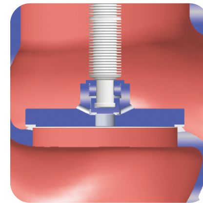
阀瓣型号/Disc type: D10 双重阀瓣设计，第二个阀瓣能够缓解压力，并且便于开启和关闭 Double disc design, the second disc can relieve pressure and easy for opening and closing.
