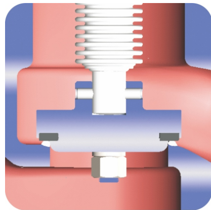
阀瓣型号/Disc type: D6 软密封表面能防止火花，且容易更换 Soft sealing surface can prevent sparks, and easy for replacement
