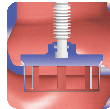
阀瓣型号/Disc type: D12 窗口形状的调节阀瓣，能精准的控制流量 Window shape regulating disc, control the flow rate precisely.
