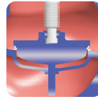
阀瓣型号/Disc type: D9 中心定位的流线型阀瓣可以防止水锤和降低噪音 Streamline disc with central locate structure can prevent water hammer and lower noise.
